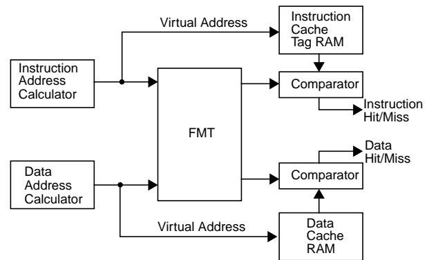
Figure 4 Address Translation During Access
